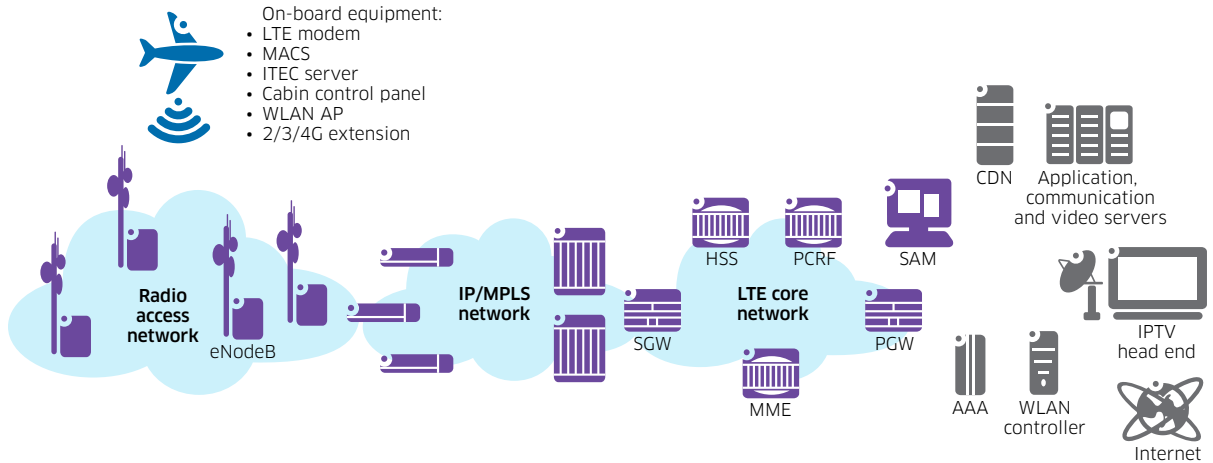
Figure 2. A2G end-to-end architecture
