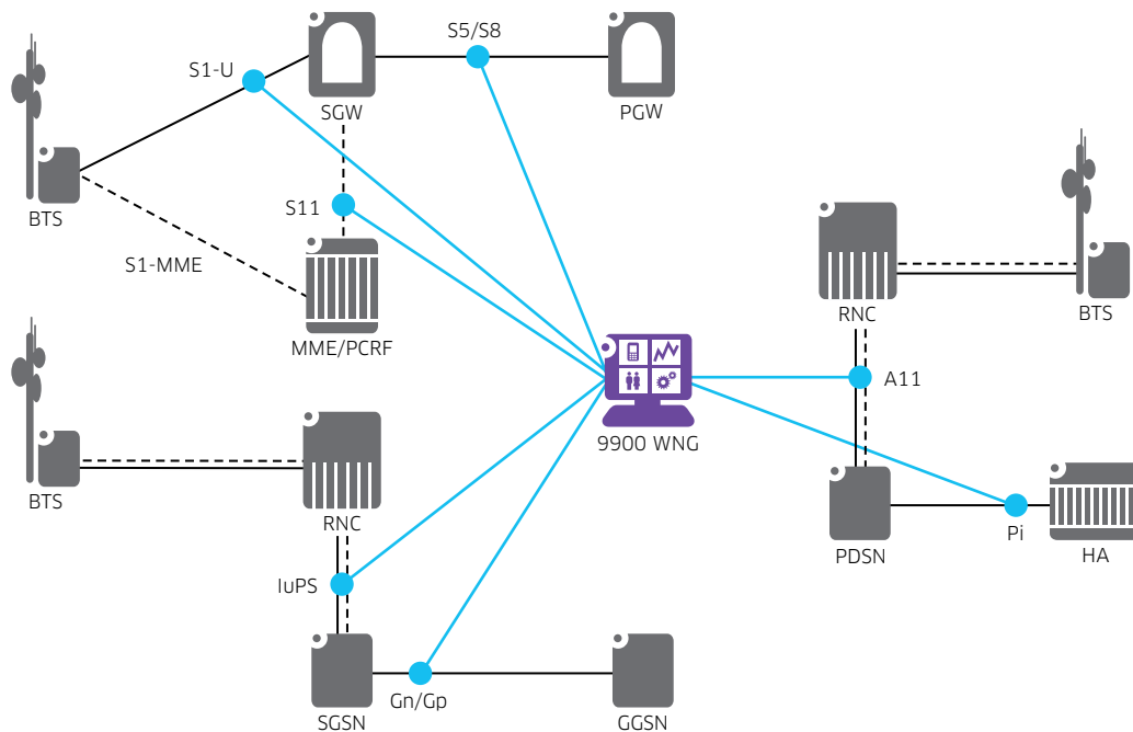
Figure 1. Alcatel-Lucent 9900 Wireless Network Guardian deployment architecture
