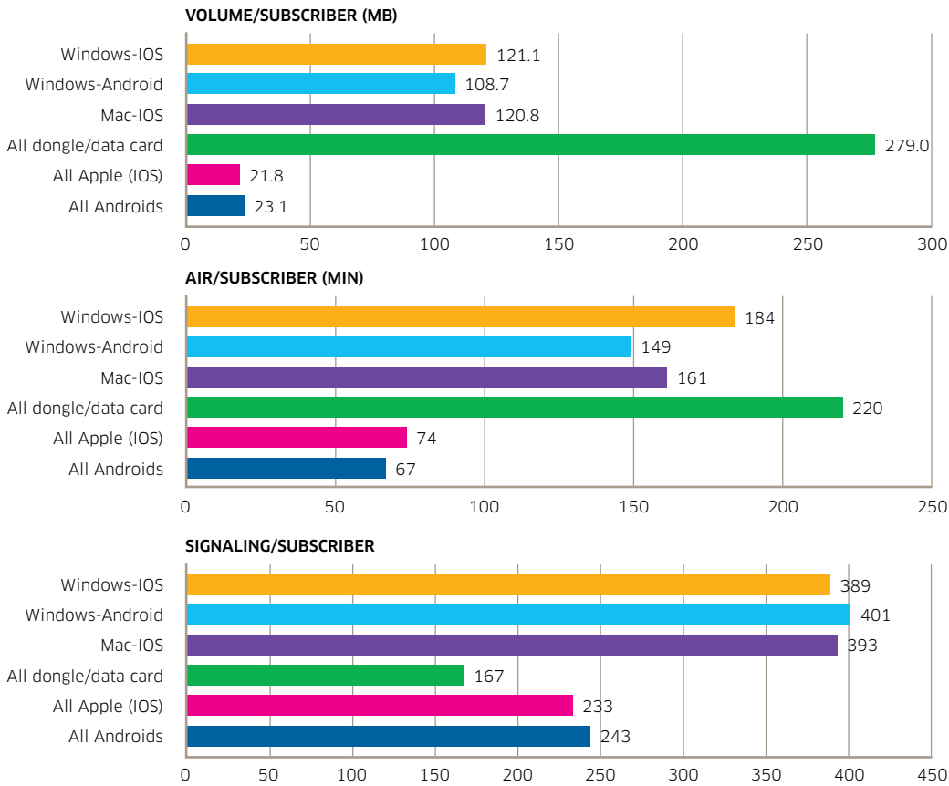
Figure 4. Alcatel-Lucent 9900 WNG reports - Top devices as they relate to volume, signaling and airtime per subscriber in the wireless network
